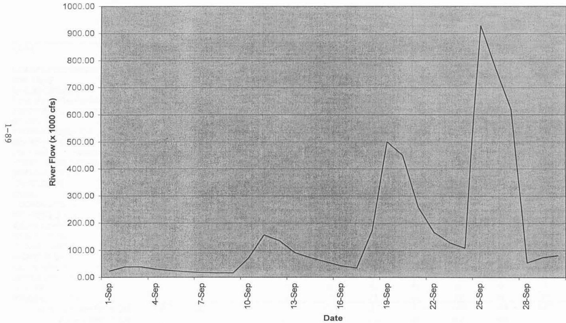
Figure 5. Plot of River Flow (x 1000 cfs) at the USGS Harrisburg Station (#01570500) on the Susquehanna River, September 2004.
