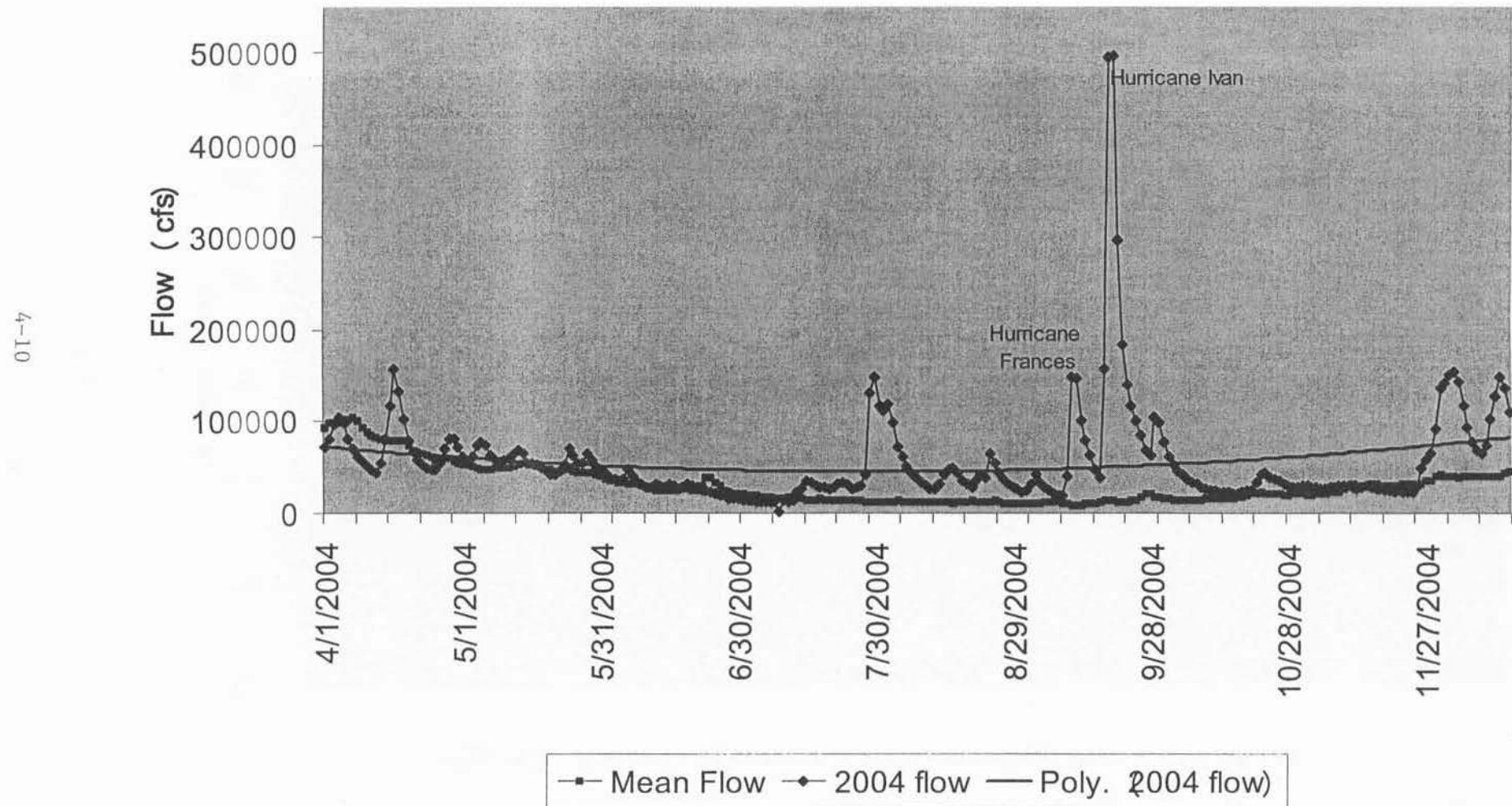
Figure 3. Susquehanna River flow at Marietta, 2004 and 72-year mean.
