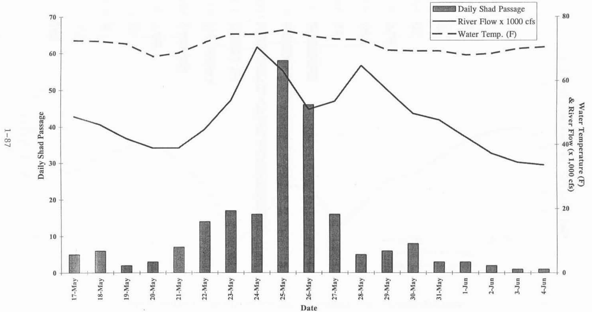
Figure 3. Plot of River Flow (x 1000 cfs) & Water Temperature (F) in Relation to the Daily American Shad Passage at the York Haven Fishway in Spring 2004
