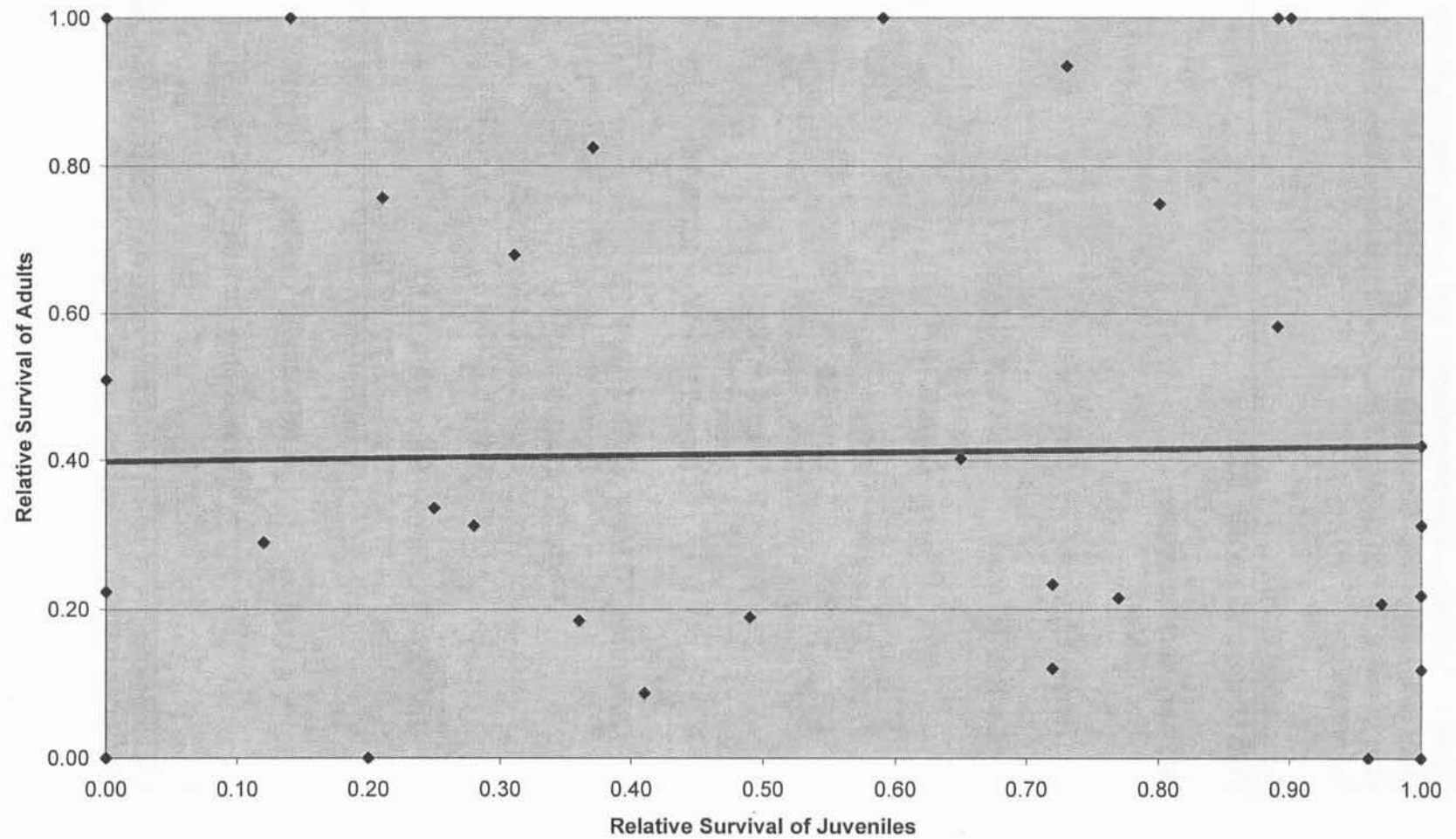
Figure 3. Stocking site/cohort specific relative survival of juvenile shad vs. adult shad, Susquehanna River, 1995-1999.
