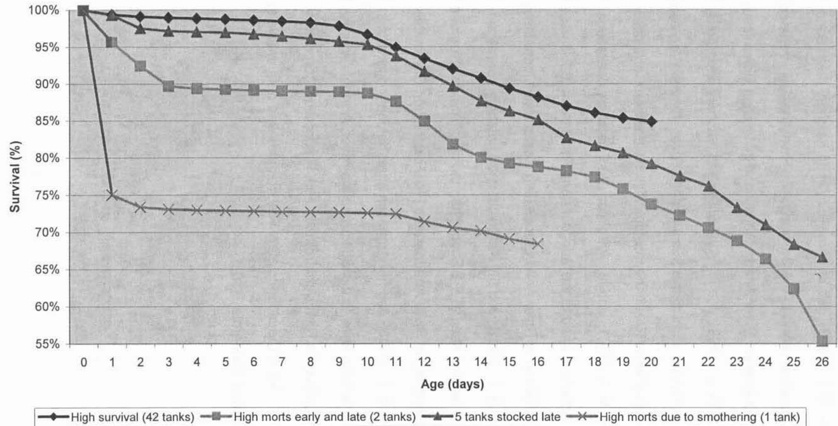
Figure 1. Survival patterns for American shad larvae reared at Van Dyke, 2003.
