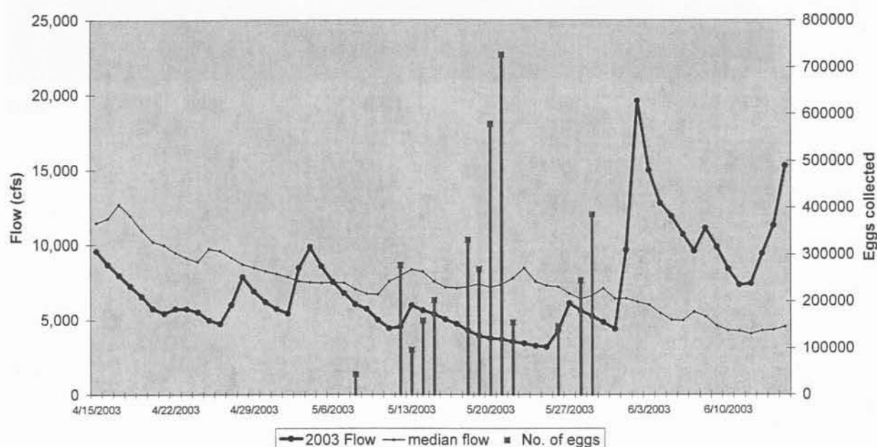
Figure 1. American shad egg collections and flow, Delaware River, 2003.
