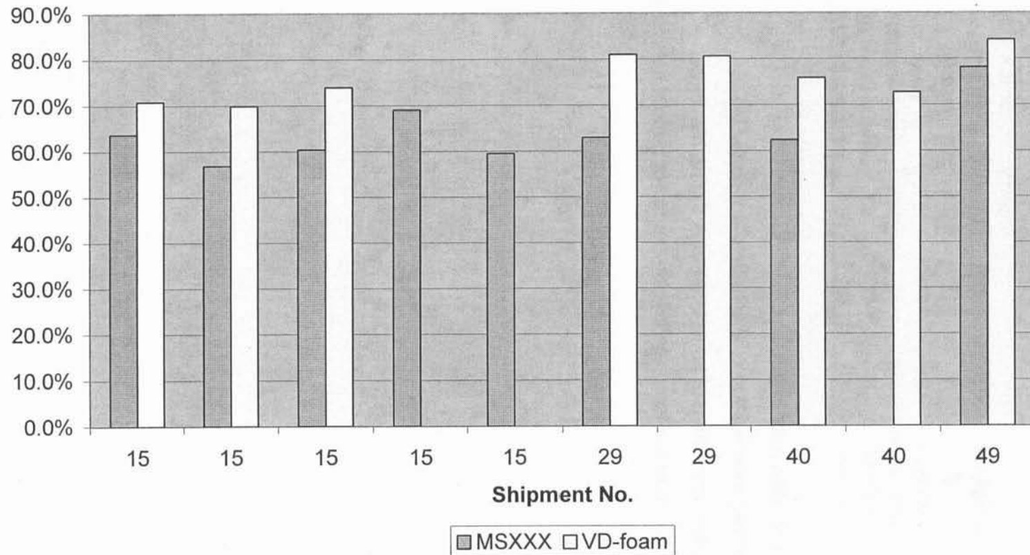
Figure 6. Percent viability of Hudson River American shad eggs incubated in MSXXX vs. VD-foam egg jar types (production lots), Van Dyke, 2003.
