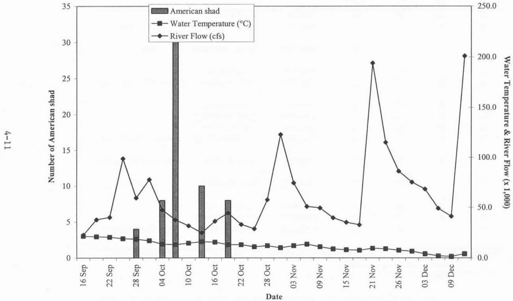
Figure 1. Water temperature and river flow in relation to the catch of juvenile American shad by lift net at Holtwood Power Station, 2003.
