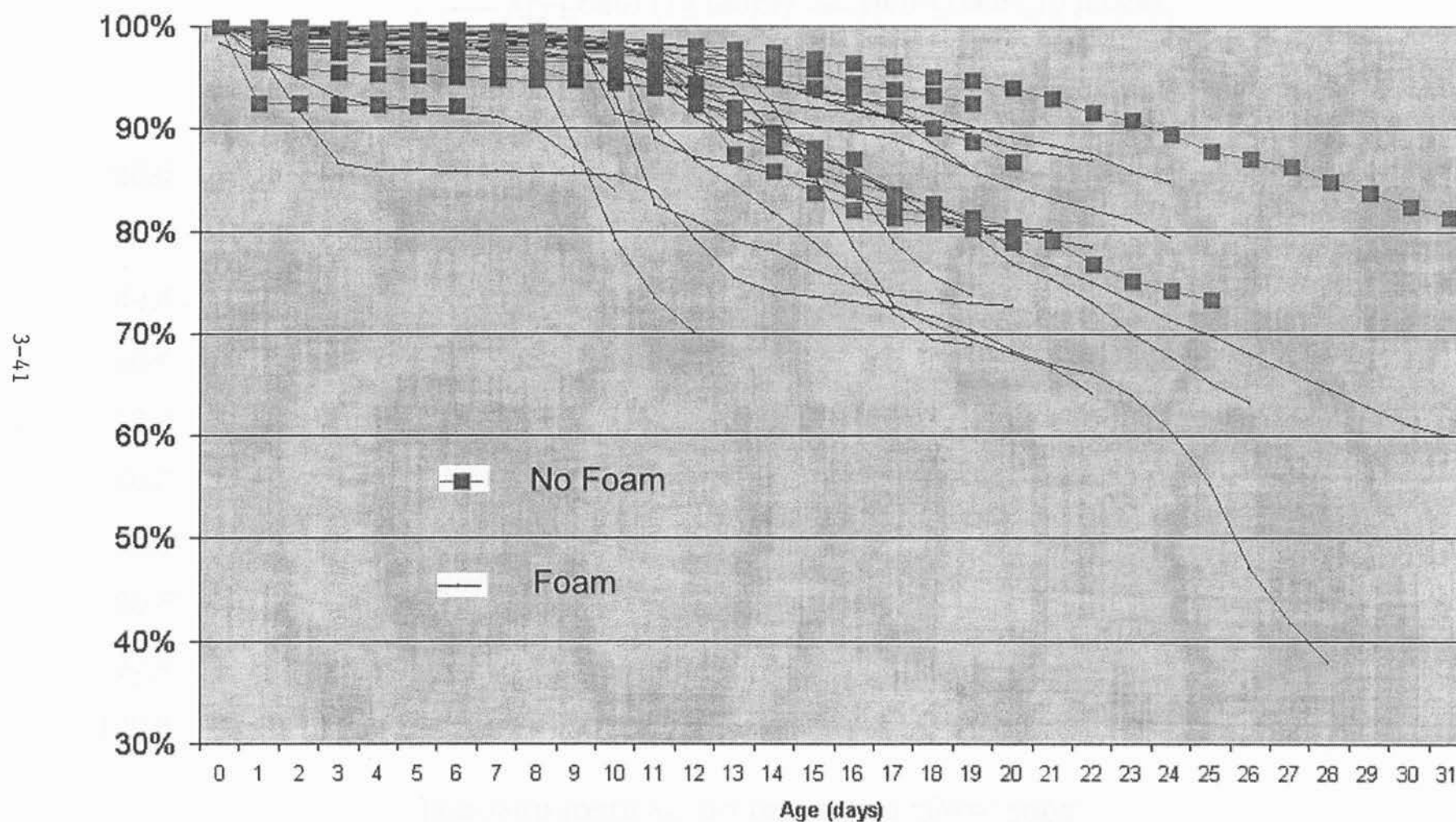
Figure 2 . Survival of larvae incubated in egg jars with foam vs no-foam, 2003.
