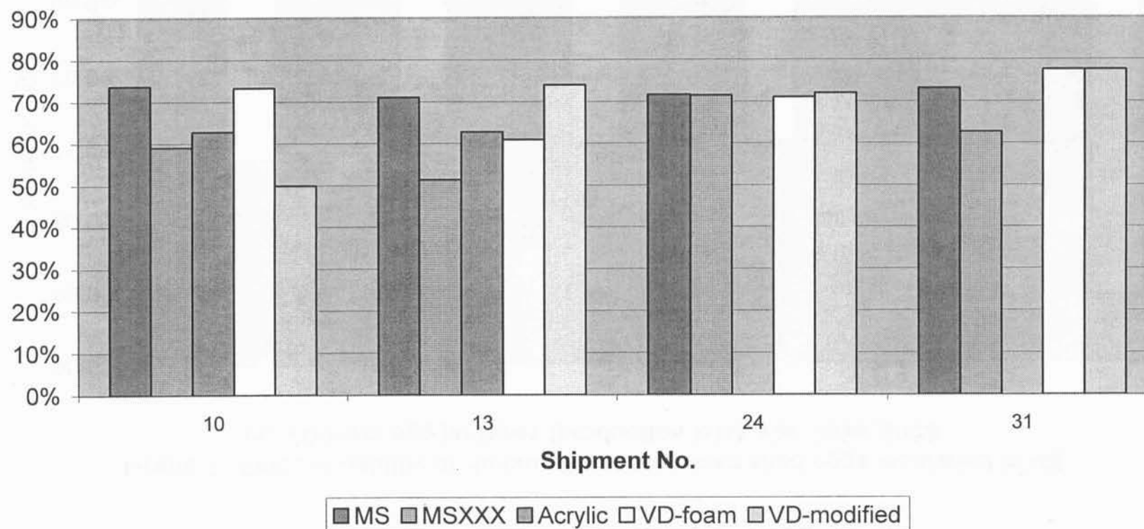
Figure 4. Percent viability of Hudson River American shad eggs incubated in various egg jar types (test lots), Van Dyke, 2003.
