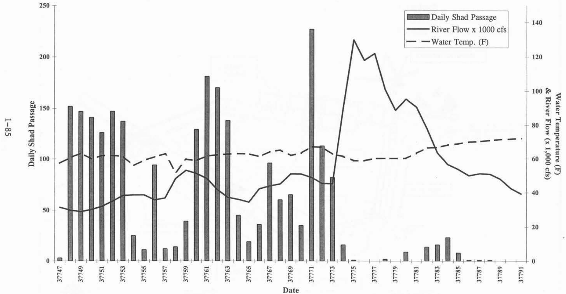
Figure 3. Plot of River Flow (x 1000 cfs) & Water Temperature (F) in Relation to the Daily American Shad Passage at the York Haven Fishway in Spring 2003
