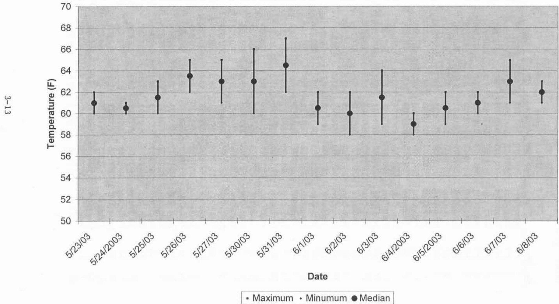
Figure 2. Maximum, minimum, and median water temperatures (F) during OTC marking of tanks that exhibited non-typical marks, Van Dyke 2003.
