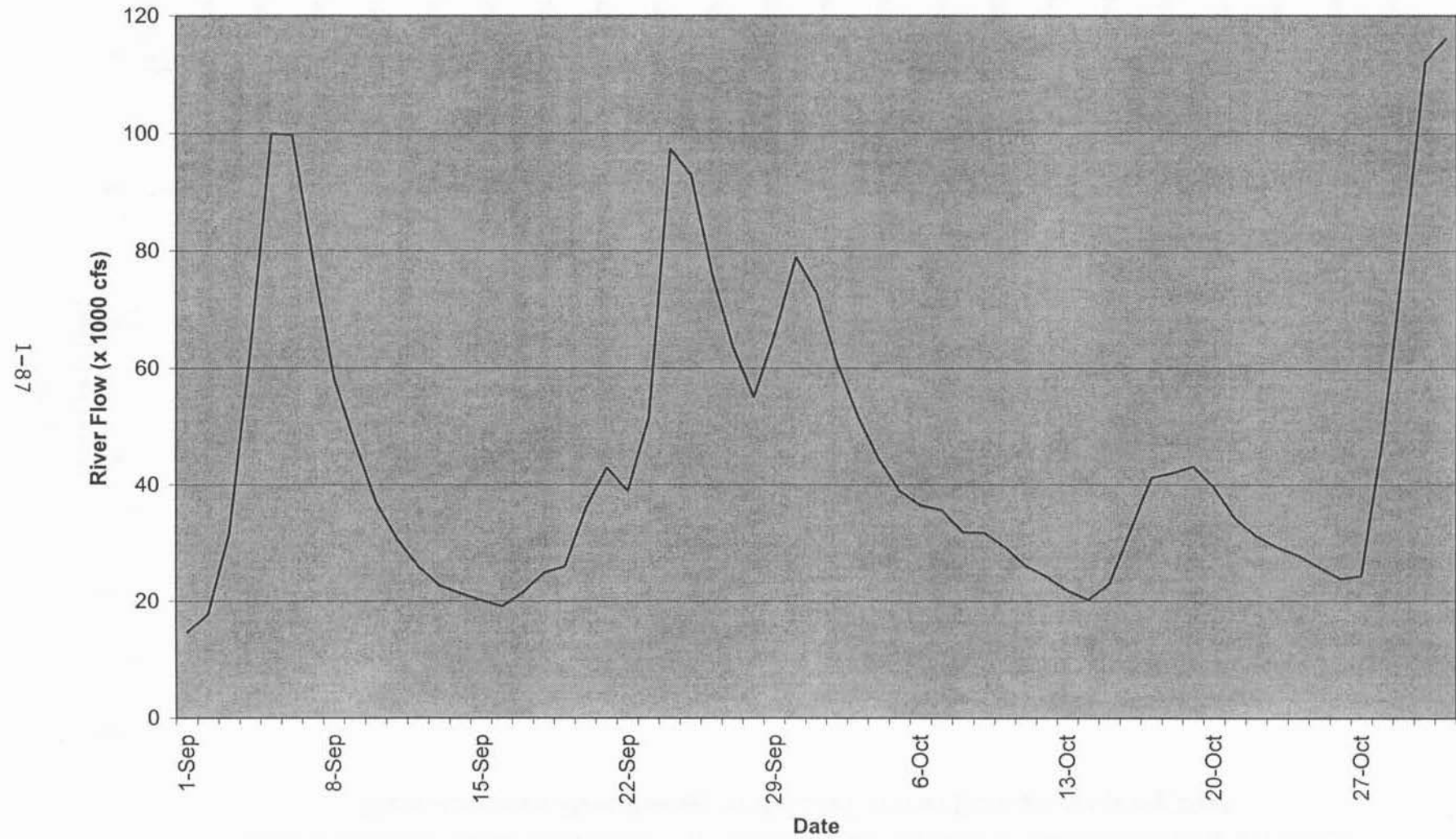
Figure 5. Plot of River Flow (x 1000 cfs), ) at the USGS Harrisburg Station (#01570500) on the Susquehanna River, September through October, 2003.
