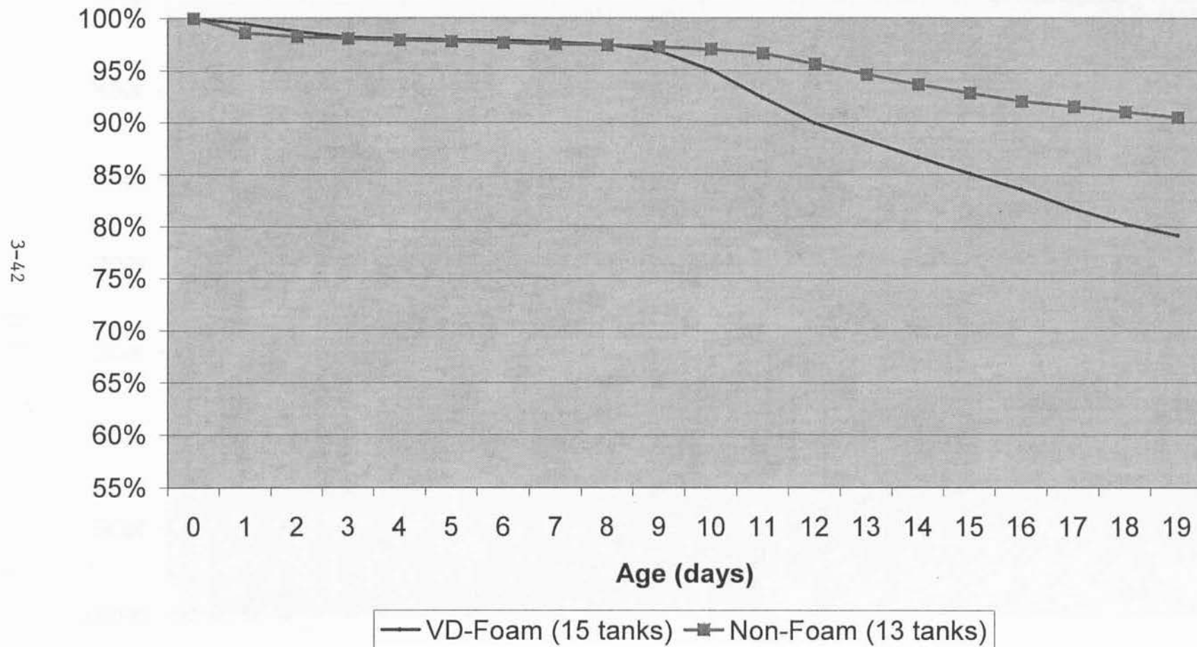
Figure 3. Mean survival for American shad larvae incubated in egg jars with foam vs. no foam, Van Dyke, 2003.
