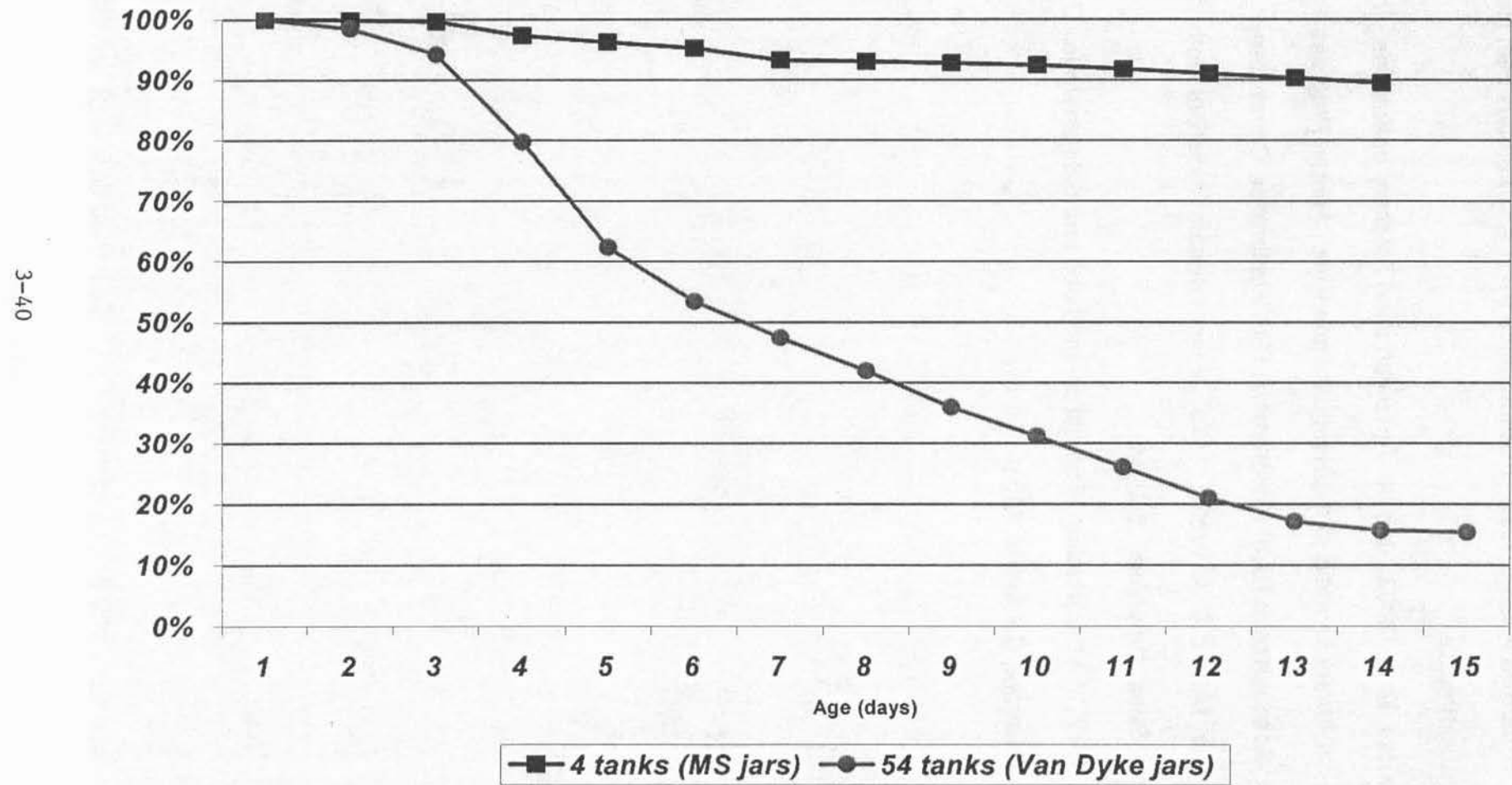
Figure 1. Survival of American shad larvae at Van Dyke, 2002.
