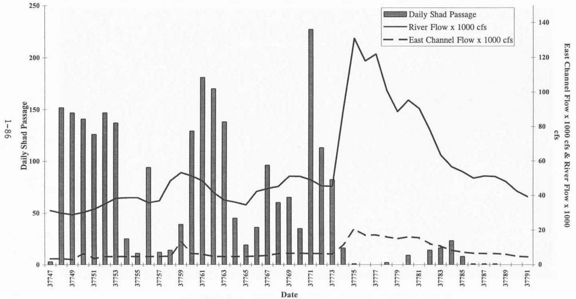
Figure 4. Plot of River Flow (x 1000 cfs) & East Channel Flow (x 1000 cfs) in Relation to the Daily American Shad Passage at the York Haven Fishway in Spring 2003
