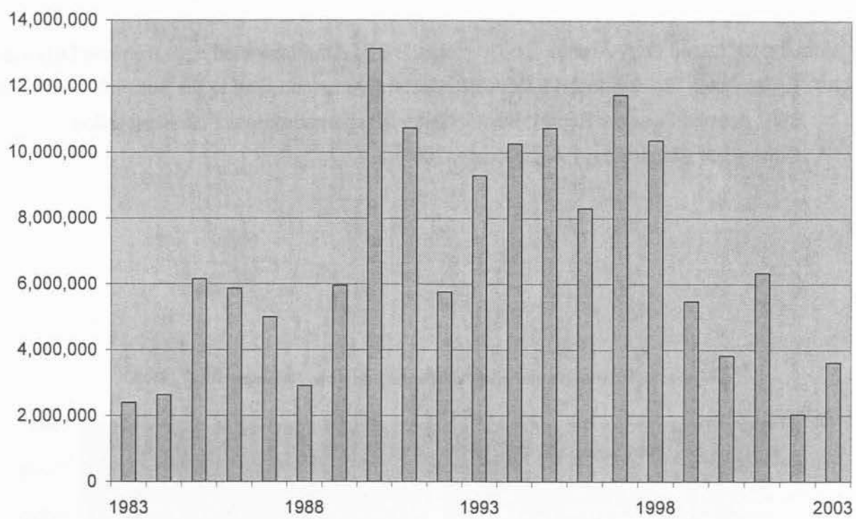
Figure 2. American shad eggs collected from the Delaware River, 1983-2003.
