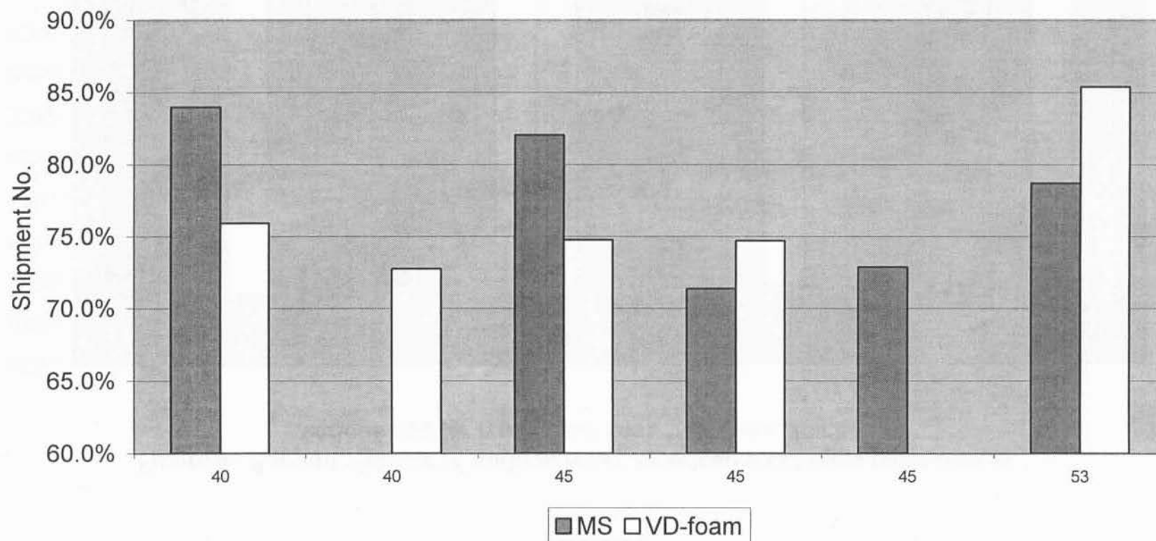
Figure 5. Percent viability of Hudson River American shad eggs incubated in MS vs. VD-foam egg jar types (production lots), Van Dyke, 2003.
