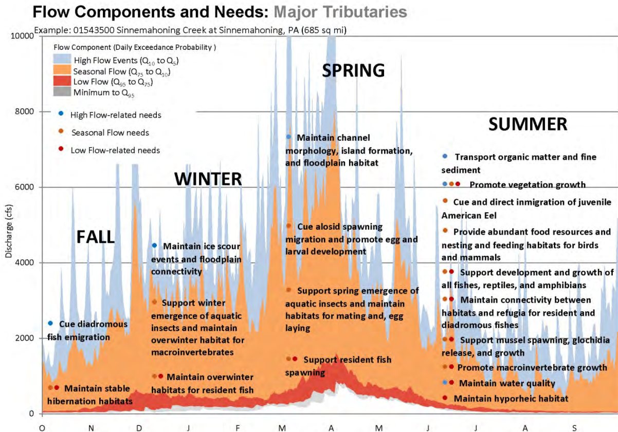
Figure 4.3 Example of flow needs associated with high, seasonal and low flows in major tributaries.
